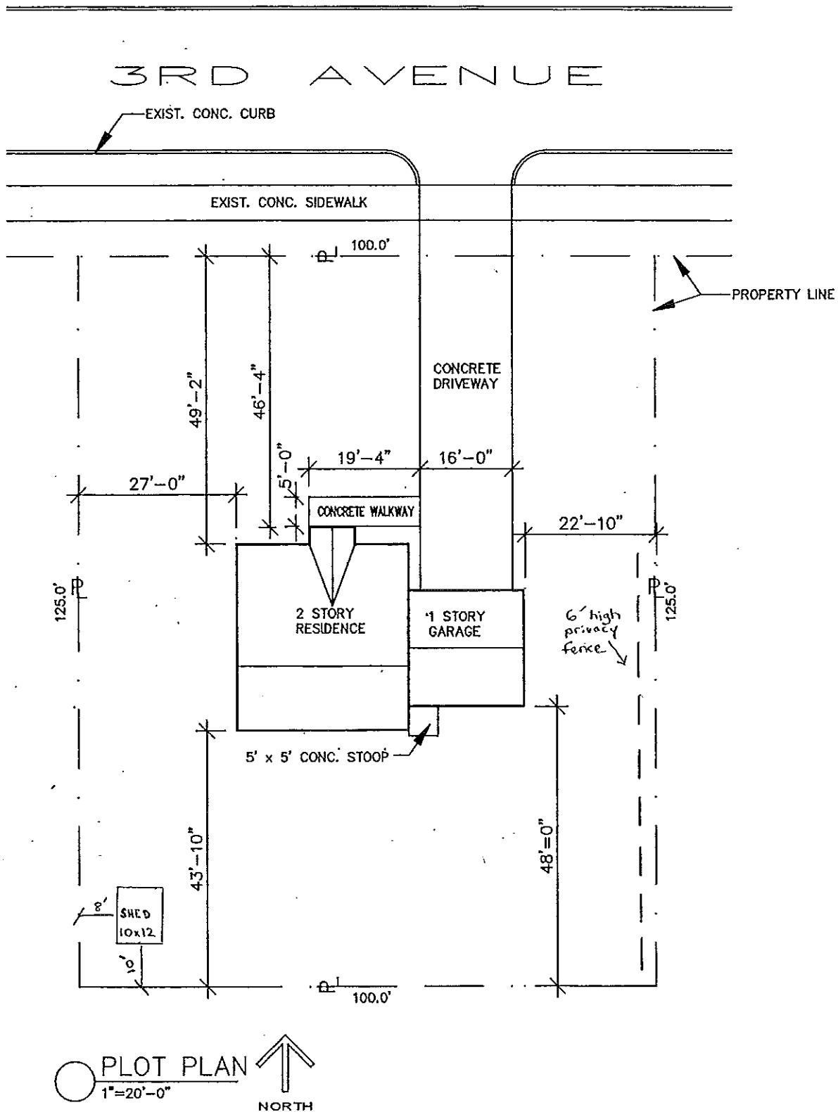
Figure 45 Rough sketch of house on site (plot plan)
